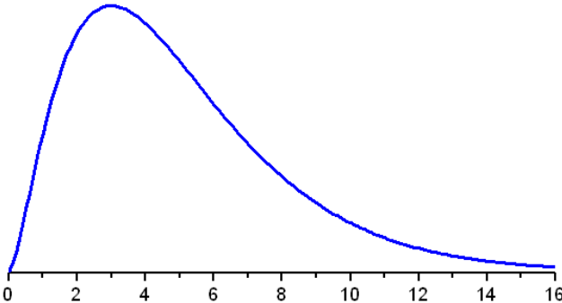
Goodness of Fit Test
